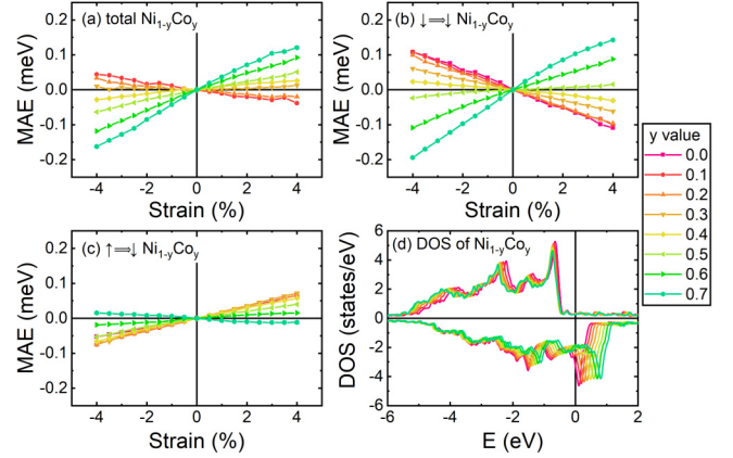
FIG. 4. Strain dependence of (a) total, (b) \downarrow \Rightarrow \downarrow , and (c) \uparrow \Rightarrow \downarrow contributions to the MAE calculated from second-order perturbation analysis for \text{Ni}_{1-y}\text{Co}_y . (d) Spin-resolved density of states of fcc- \text{Ni}_{1-y}\text{Co}_y .
