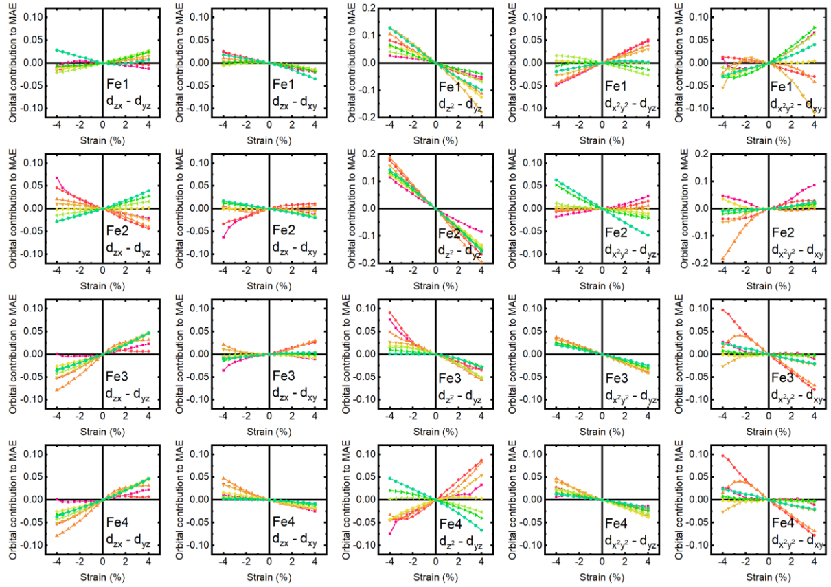
FIG. S3. Strain dependence of the \downarrow\Rightarrow\downarrow normalized orbital contribution to the MAE calculated from second-order perturbation analysis of (\text{Fe}_{1-x}\text{Co}_x)_4\text{N} , divided by atomic site (from top to bottom: Fe1; Fe2; Fe3; Fe4) and orbital combination (from left to right: d_{zx} - d_{yz} ; d_{zx} - d_{xy} ; d_{z^2} - d_{yz} ; d_{x^2-y^2} - d_{yz} ; d_{x^2-y^2} - d_{xy} ).
