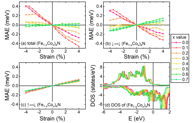
FIG. 2. Strain dependence of (a) total, (b) \downarrow \Rightarrow \downarrow , and (c) \uparrow \Rightarrow \downarrow contributions to the MAE calculated from second-order perturbation analysis for (\text{Fe}_{1-x}\text{Co}_x)_4\text{N} . (d) Spin-resolved density of states of (\text{Fe}_{1-x}\text{Co}_x)_4\text{N} .
