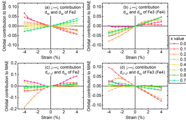
FIG. 3. Strain dependence of the \downarrow \Rightarrow \downarrow normalized orbital contribution to the MAE of the (\text{Fe}_{1-x}\text{Co}_x)_4\text{N} calculated from second-order perturbation analysis for (a) d_{xz}-d_{yz} of Fe2, (b) d_{xz}-d_{yz} of Fe3 (Fe4), (c) d_{x^2-y^2}-d_{xy} of Fe2, and (d) d_{x^2-y^2}-d_{xy} of Fe3 (Fe4).
