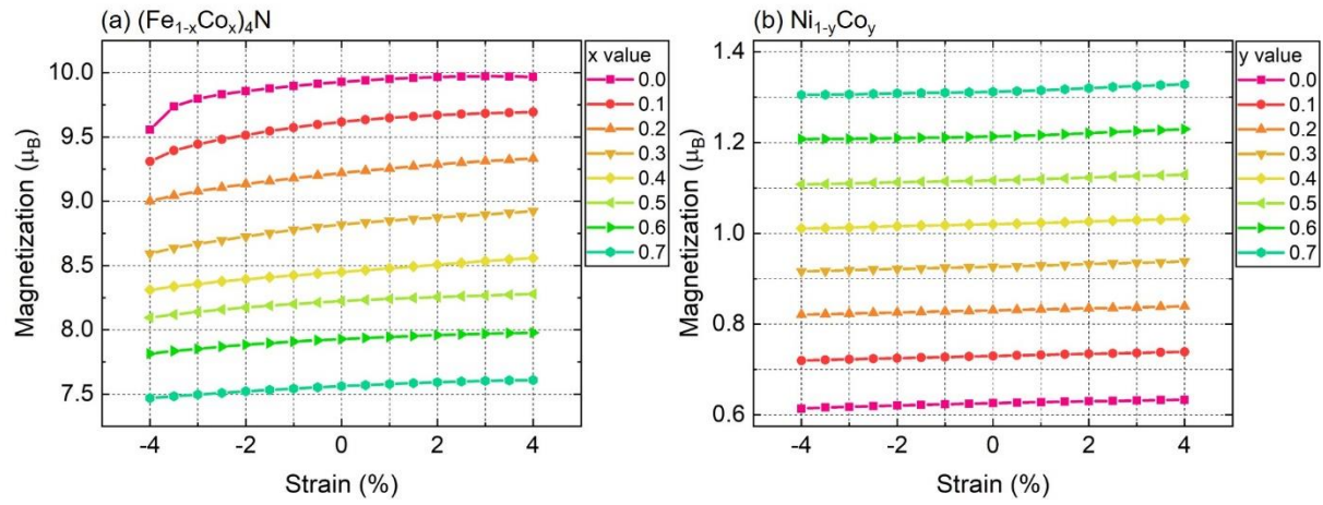
FIG. S1. Strain dependence of magnetization for (a) (\text{Fe}_{1-x}\text{Co}_x)_4\text{N} with varying x values and (b) \text{Ni}_{1-y}\text{Co}_y with varying y values. Gridlines are added for clarity.
