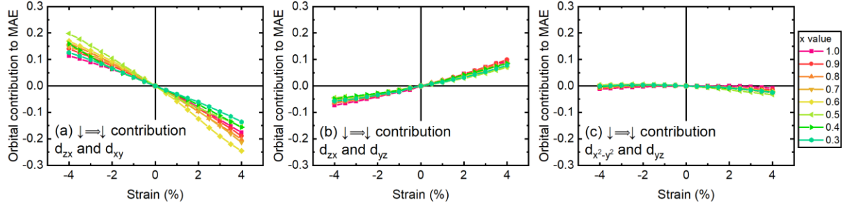
FIG. S4. Strain dependence of the \downarrow\Rightarrow\downarrow normalized orbital contribution to the MAE calculated from second-order perturbation analysis of (a) d_{zx} - d_{xy} , (b) d_{zx} - d_{yz} , (c) d_{x^2-y^2} - d_{yz} of \text{Ni}_{1-y}\text{Co}_y
