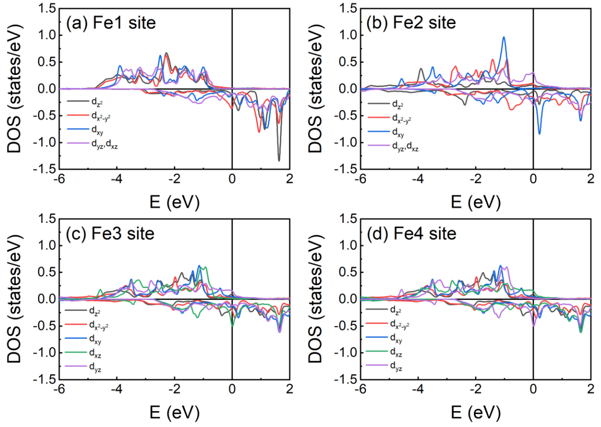
FIG. S2. Partial density of states for (a) Fe1, (b) Fe2, (c) Fe3, (d) Fe4 sites of tetragonally distorted Fe 4 N
